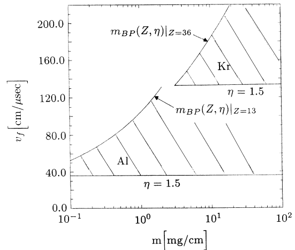
FIG. 1. Two shaded regions for aluminum and krypton defined by the boundary curves \eta = 1.5 and m = m_{BP}(\eta) are shown. In these regions, efficient conversion of z-pinch kinetic energy into K -shell emission is predicted to occur.
